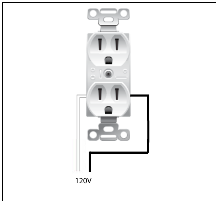
Figure 69: C72I Receptacle Wiring
