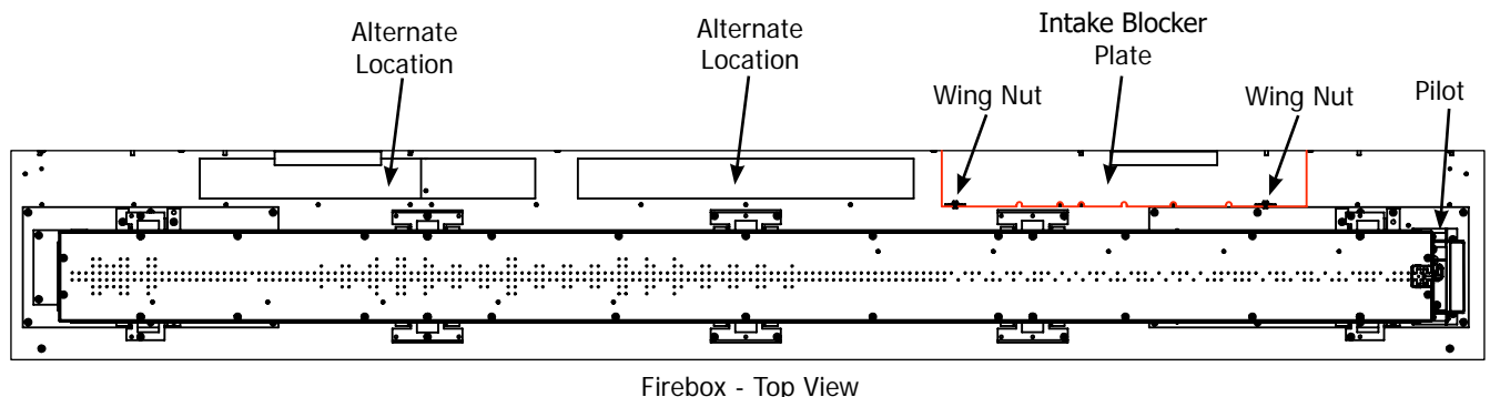
Figure 61: Intake Blocker Plate
