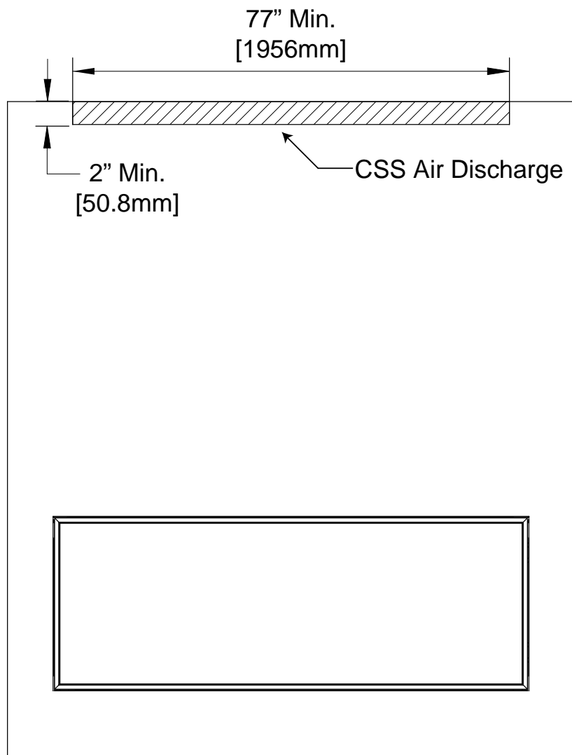
Figure 34: CSS Front Outlet
