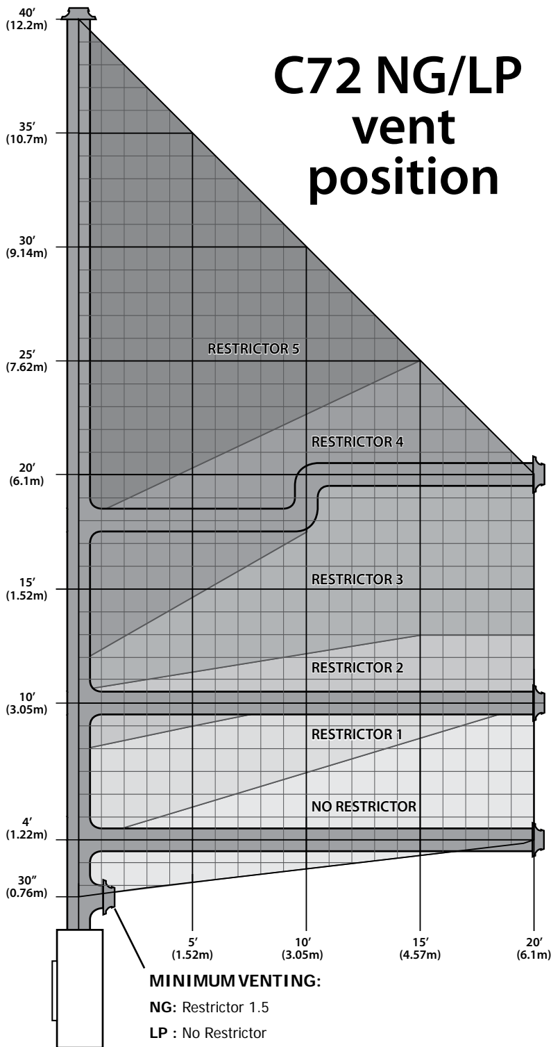
Figure 59: NG/LP Vent Graph
