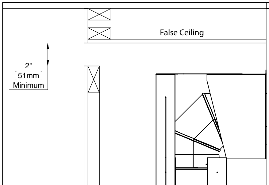
Figure 36: False Ceiling
